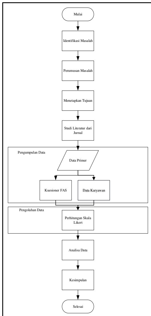
Gambar 1. Flowchart Penelitian
