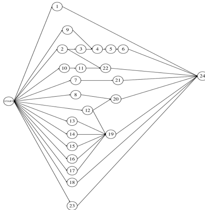
Figure 2. Precedence Diagram
