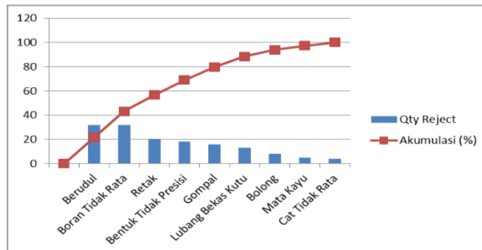
Gambar 2. Pareto Diagram
