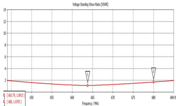
Figure 4. VSWR of Yagi-Uda Antenna
