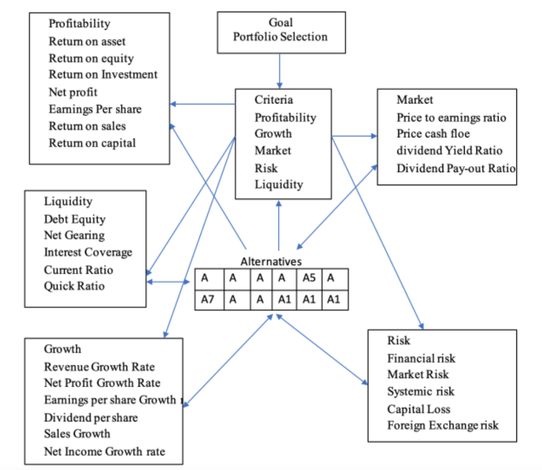
Shariah Portfolio Selection Model
