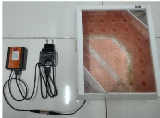
Figure 1. ECCT device for animal study. The size of the cage is 23 cm × 18 cm × 19 cm. The electrodes are attached to the acrylic wall of the cage with opposite polarity facing each other to produce multiple field directions.
