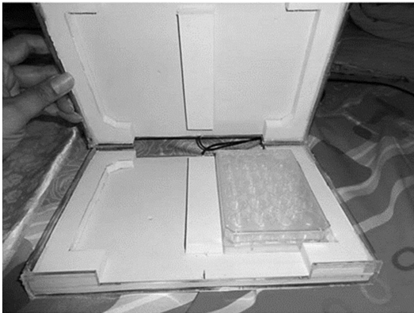
Figure 1. Capacitive electrodes as electrical field generator. A microplate was flanked between two capacitive electrodes that were connected to low intensity oscillator to generate the alternate electric field
