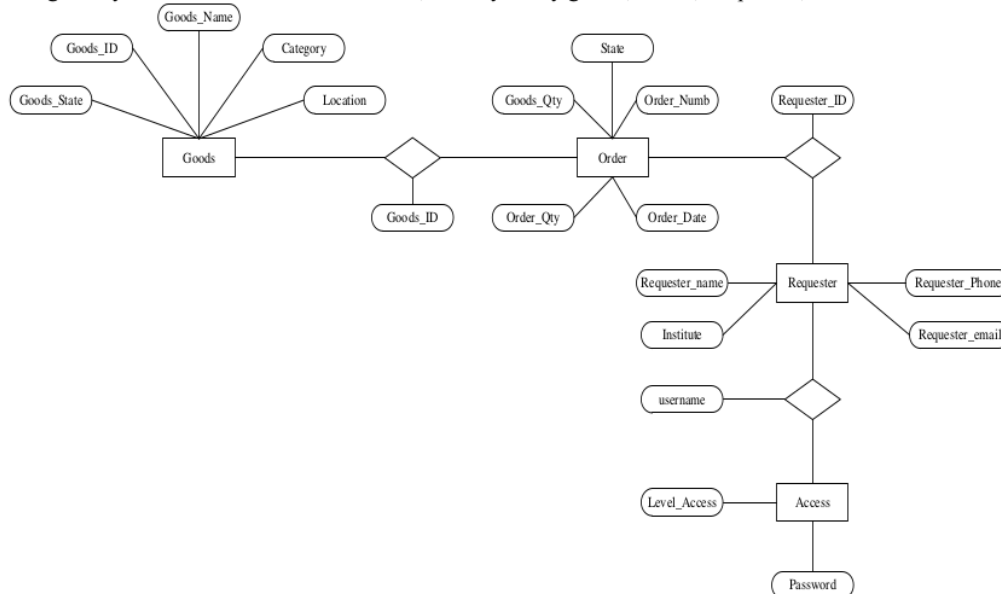
Figure 8. ERD Warehouse Information System of Public Relations and PMB
