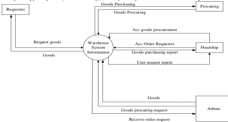
Figure 5. DFD Level 0 Design of Information Systems for Promotion Bureau Warehouse
