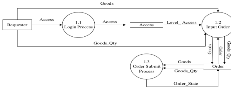
Figure 7. DFD Level 2 Request by User
