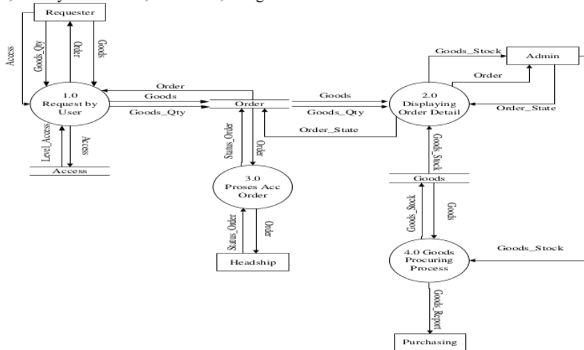
Figure 6. DFD Level 1 Information Systems Design
