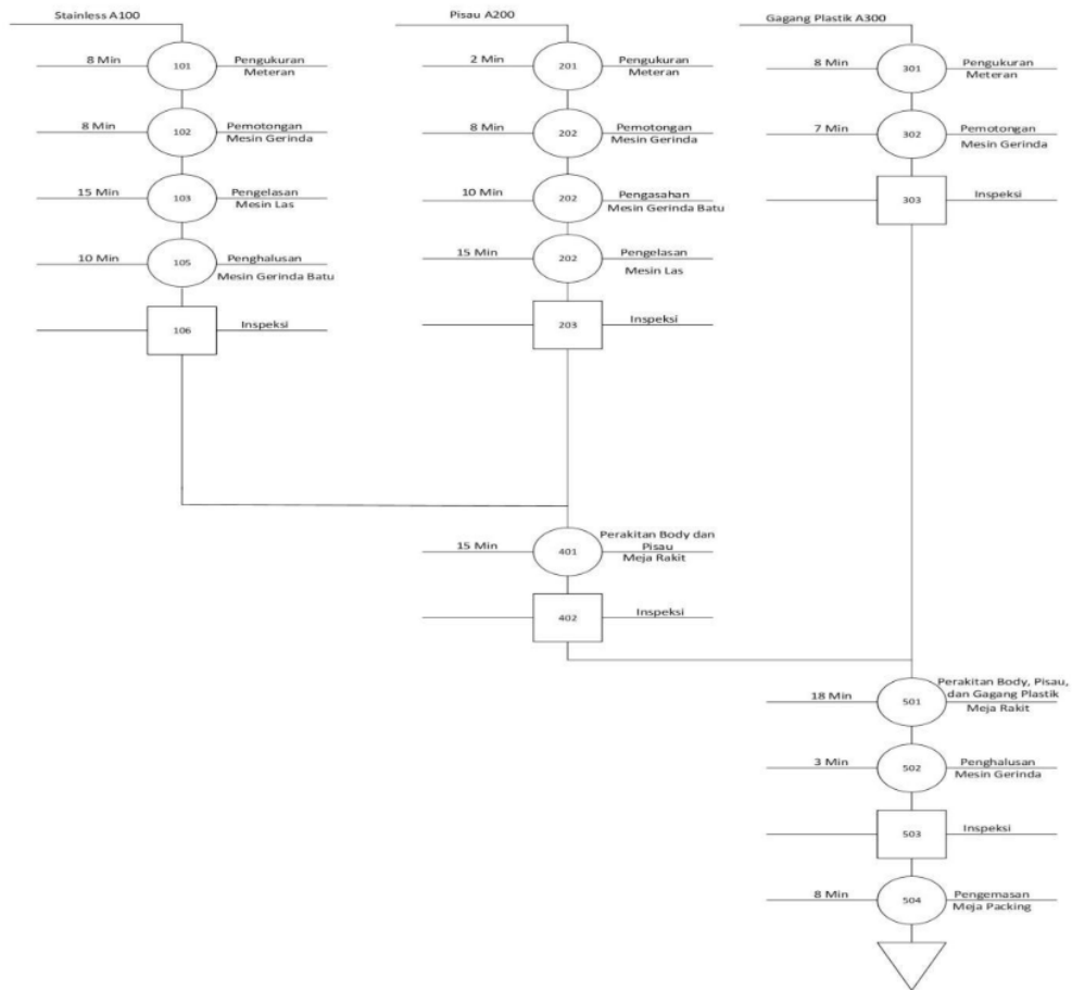
Gambar 2. Operation Process Chart
