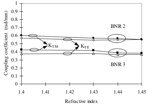
Figure 5. Variation of the coupling coefficient of two different directional couplers with the refractive index of the upper cladding layer
