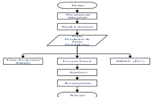
Gambar 1 Flowchart Penelitian
