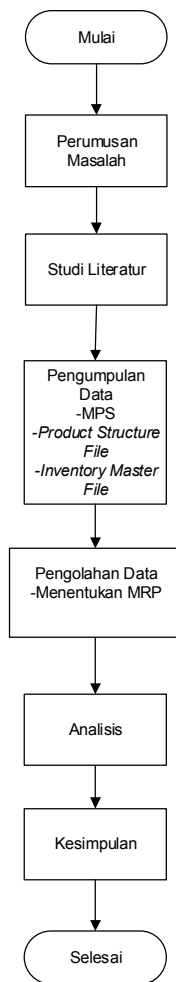
Gambar 1 Flowchart Penelitian
