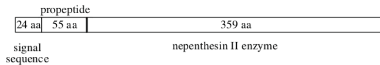
Figure 1. Illustration of the prepro-form of nepenthesin II, composed of 438 amino acids, including 24 residues putative signal sequence, 55 residues putative propeptide, and 359 residues enzyme.
